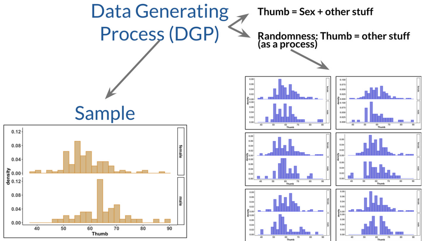
Figure 1. Sample R plots students created to explore the distribution triad. When exploring variation, students focus on connecting two types of distributions (sample and DGP), representing possible explanations with informal models instantiated as word equations, and exploring those explanations with data visualizations (e.g., faceted histograms). They further explore randomness as a DGP by actually generating data with a random process (using an R function, shuffle ) which breaks any relationship between the explanatory variable (Sex) and the outcome (Thumb) by shuffling which Thumb length goes with which Sex group. The histograms in blue visualize six independent examples of shuffled data. Does the empirical sample look similar to these shuffled samples? Considering this question puts students on the path to understand the logic of sampling distributions, far ahead of their formal introduction.
