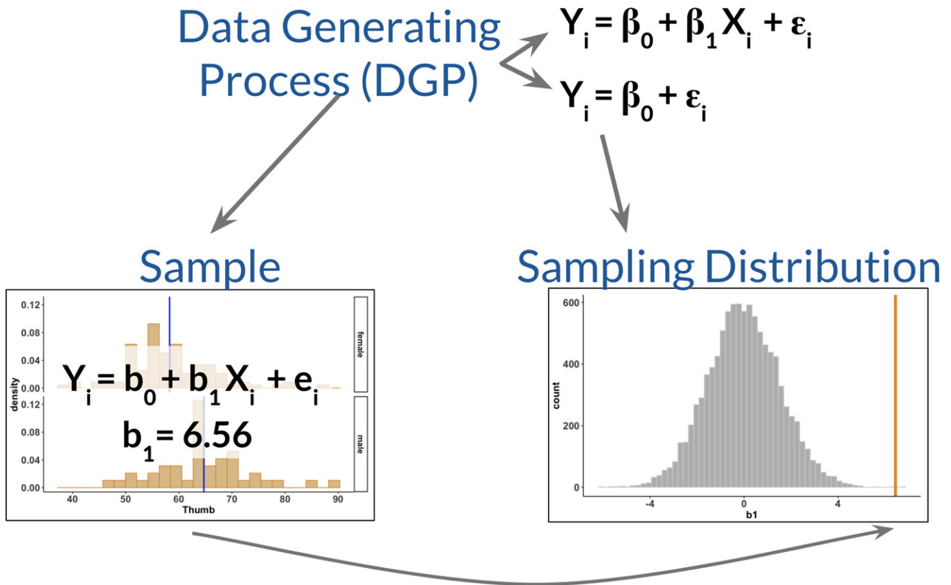
Figure 3. Evaluating models. When “evaluating models,” students go beyond the best fitting parameter estimates in their models. They consider how those parameter estimates could potentially vary depending on different DGPs. Students connect the shuffling (randomization) and resampling (bootstrapping) they have done with building up sampling distributions of particular parameter estimates such as the b_1 values (pictured here), or PRE or F.
